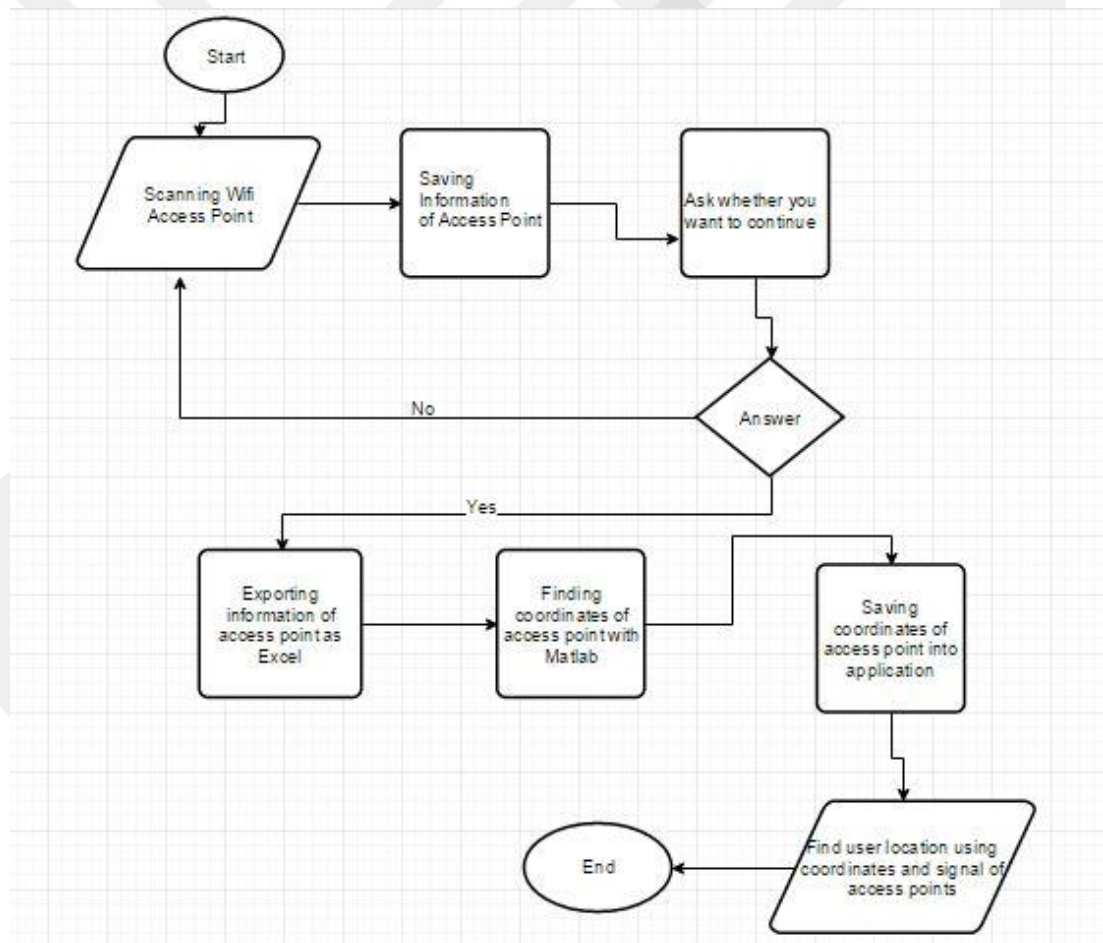
Figure 4.1: Flow chart of indoor positioning system
