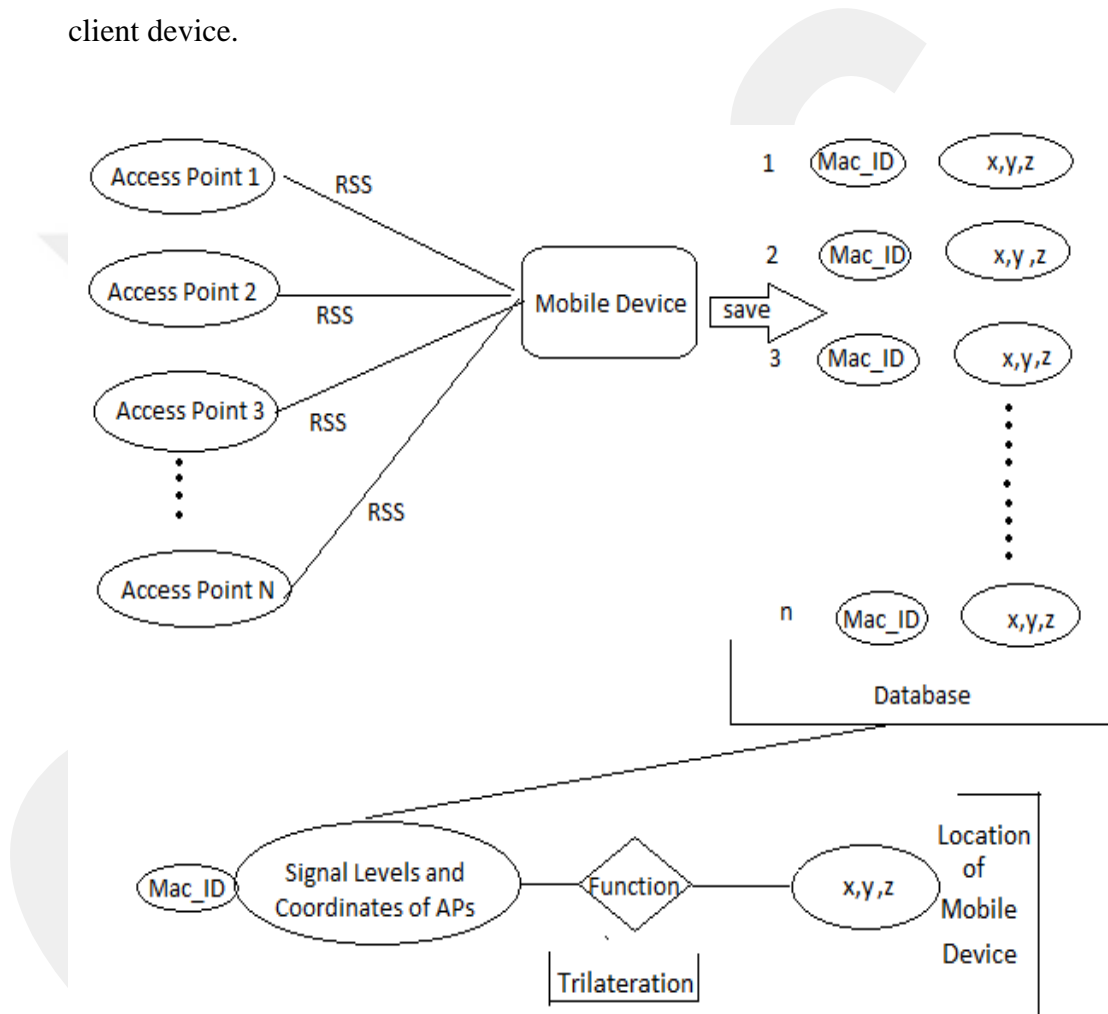
Figure 3.7: The working principle of application
