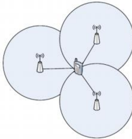
Figure 3.5: Location determination with time of arrival (ToA) method [8]
