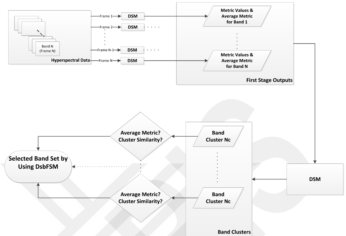
Figure 3.10: DSbFSM Algorithm
