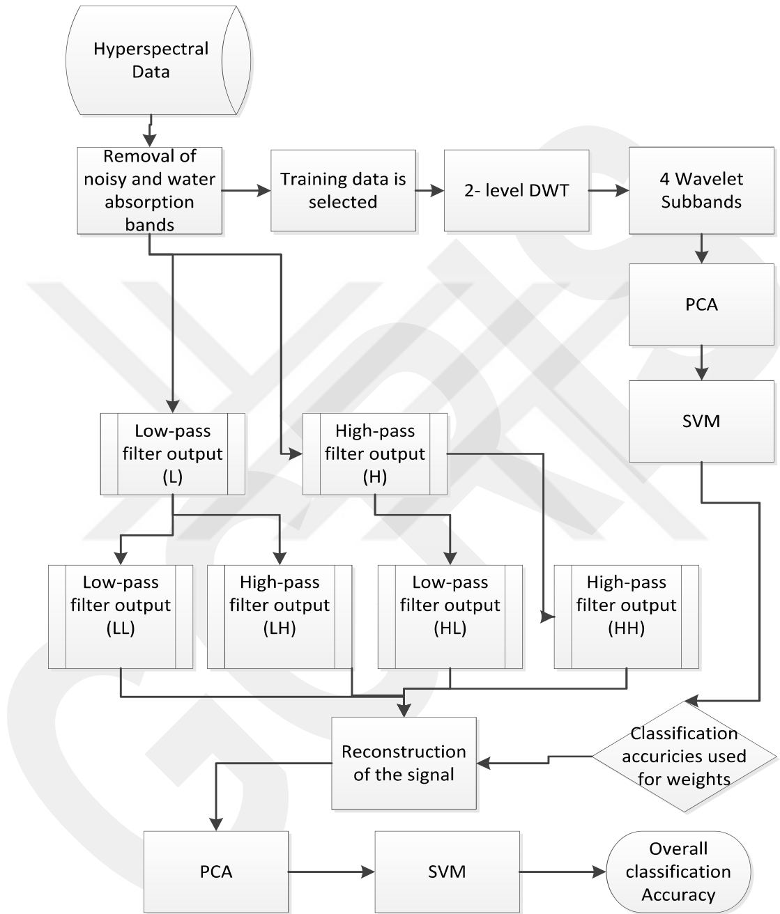
Figure 3.2: Sub-band Decomposition Based Supervised Feature Extraction Algorithm
