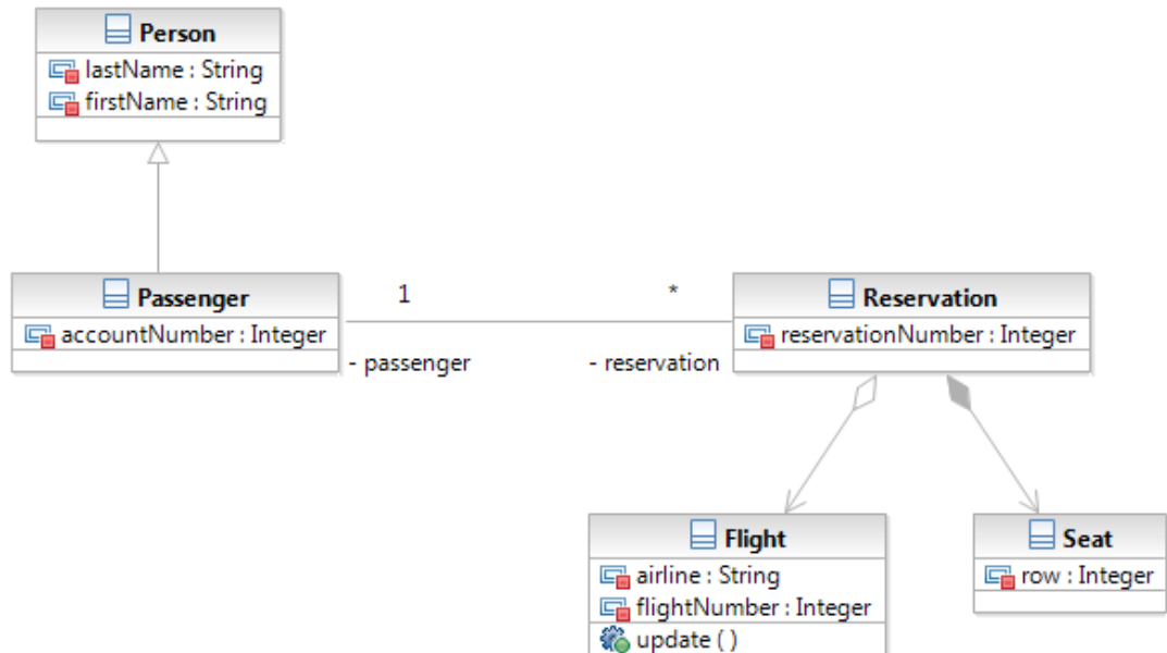
Figure 2.1 Class Diagram
