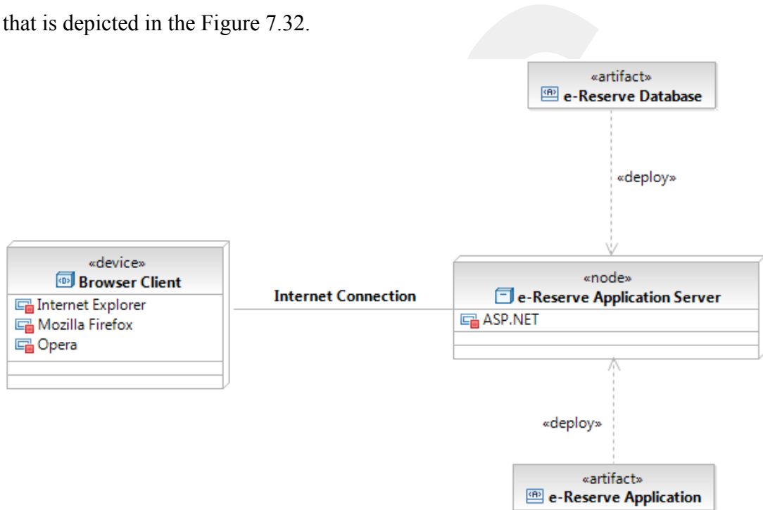
Figure 7.32 Deployment Model
