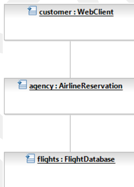
Figure 2.2 Object Diagram
