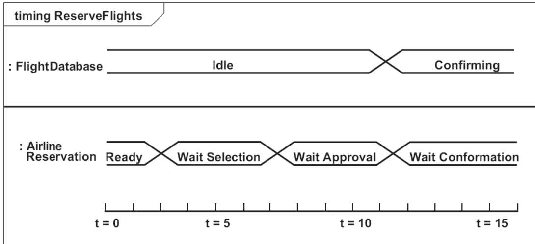
Figure 2.13 Timing Diagram
