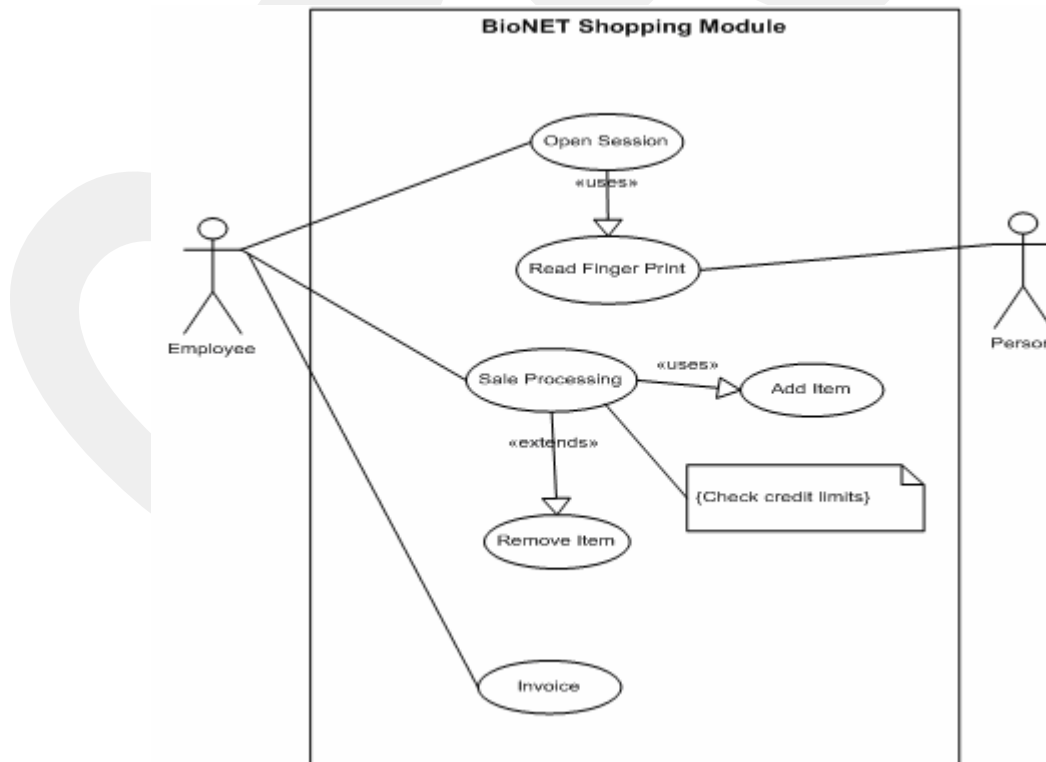
Figure 22. Use Case Diagram of Shopping Module
