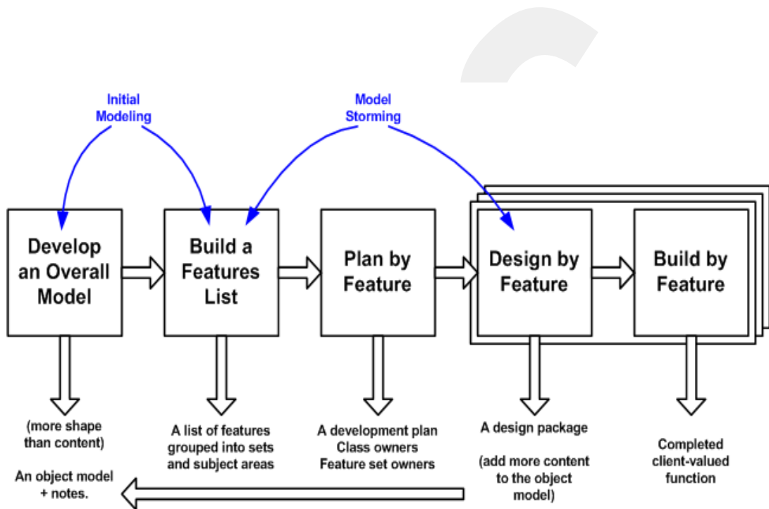
Figure 5. The FDD Project Lifecycle
