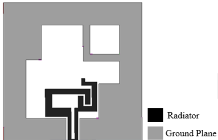
Figure 114 The structure of second update CPSSA
