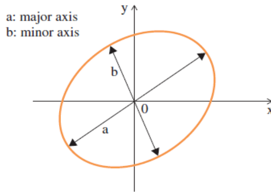
Figure 24 2-D elliptical polarization trace
