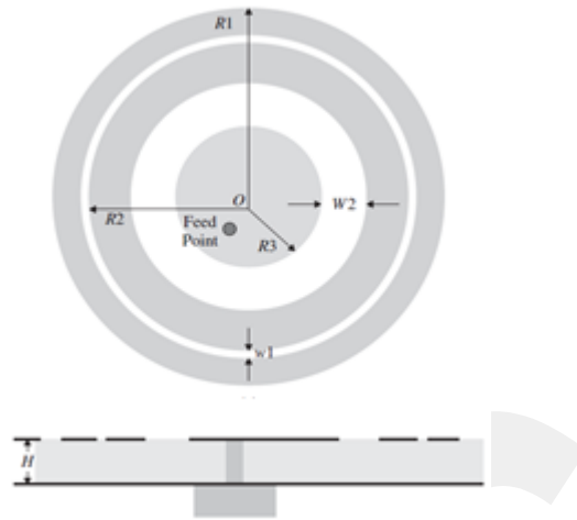
Figure 59 The geometry of the dual band CP annular ring antenna [95]
