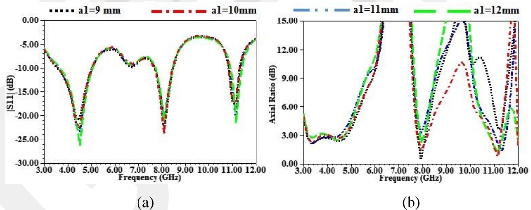
Figure 96 The effect of a_1 on antenna performance (a) |S_{11}| , (b) AR
