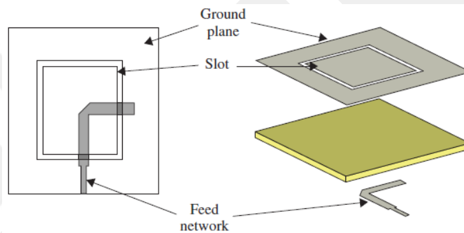
Figure 53 Circular slot antenna fed by an L-shaped fed [1]
