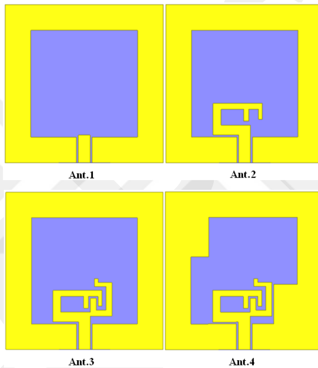
Figure 93 The steps to perceive the triple band CPSSA
