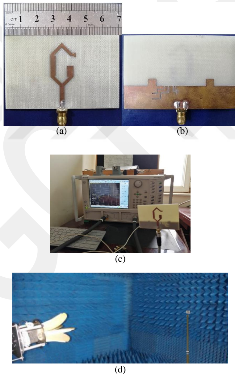
Figure 88 The fabricated of the modified antenna (a) Top view, (b) Bottom view, (c) Under VNA test (d) Measurement of radiation in the anechoic chamber
