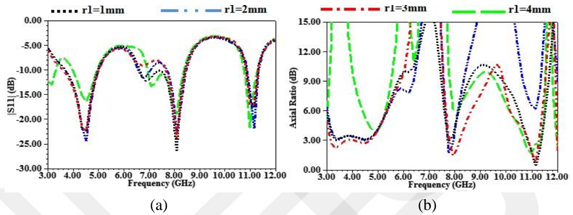
Figure 99 The effect of r_1 on antenna performance (a) |S_{11}| , (b) AR
