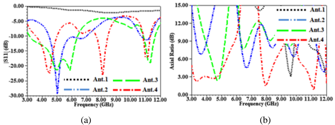
Figure 94 The response of each step of the proposed CPSSA (a) |S_{11}| , (b) AR
