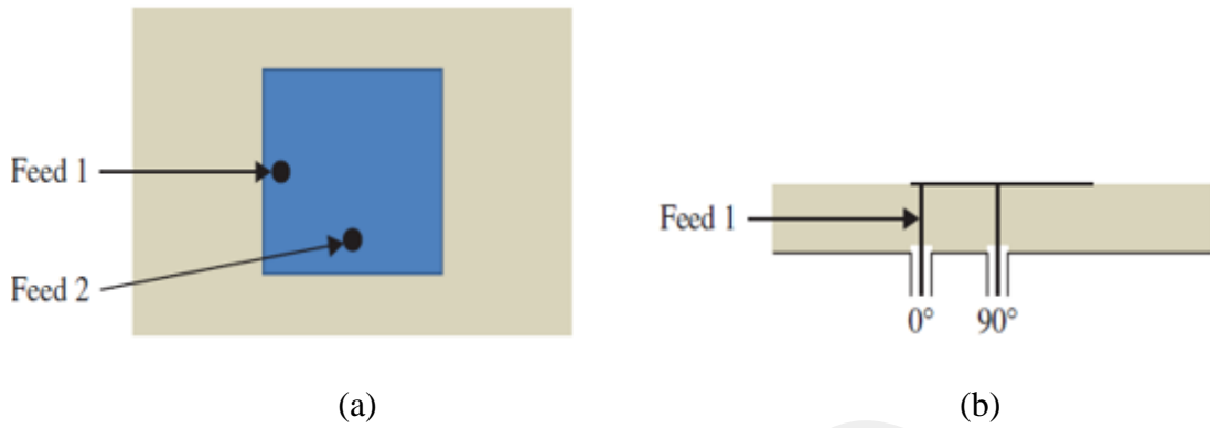
Figure 41 A probe-feed patch antenna with an external 90° phase shifter (a) Top view, (b) Side view [1]
