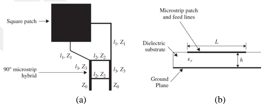
Figure 40 Microstrip line feed patch antenna with a 90^\circ hybrid (a) Top view, (b) Side view [1]
