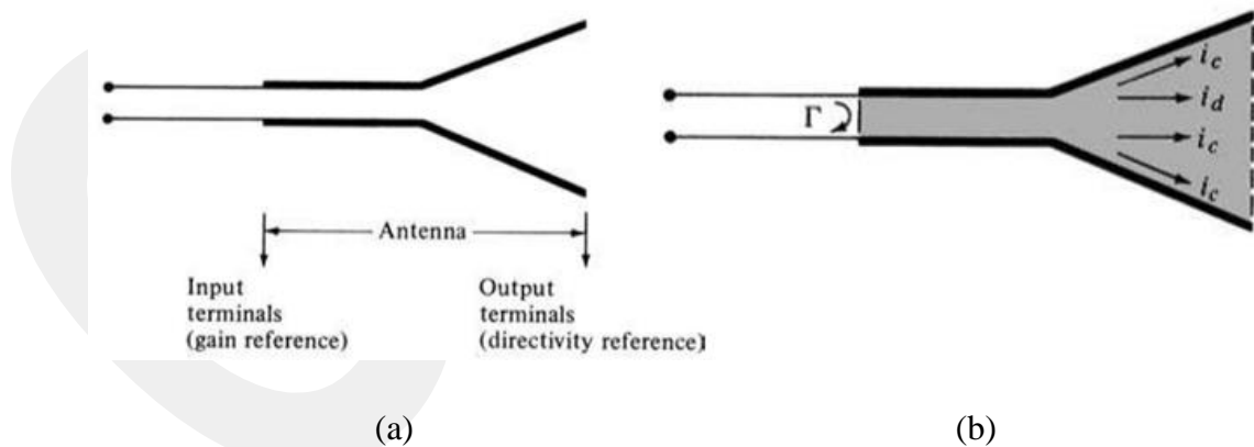
Figure 20 Reference terminals and losses of an antenna: (a) Antenna reference terminals, (b) Reflection, conduction, and dielectric losses [28].
