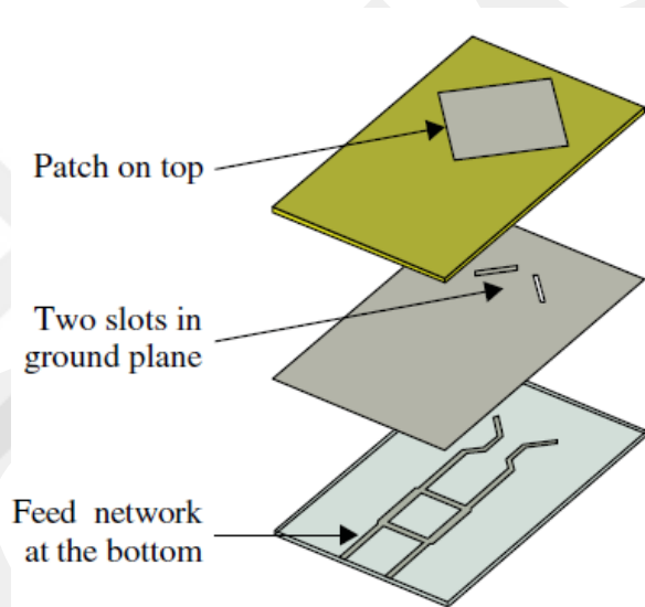
Figure 42 Slot coupled CP patch antenna (dual feed with a hybrid coupler) [1]
