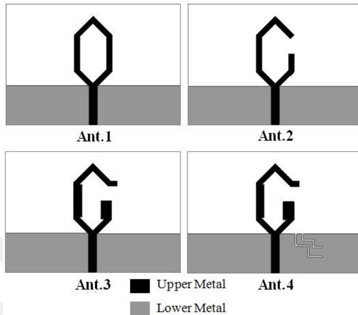
Figure 68 Steps of open loop hexagonal penta band triple sense CP antenna design
