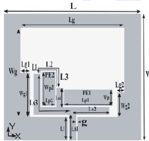
Figure 13 The geometry of wide slot dual band dual sense CP antenna with CPW-fed
