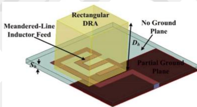
Figure 50 Dielectric resonator antenna with CP radiation [75].
