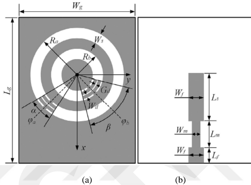
Figure 10 The geometry of capacitive load dual band dual sense CP antenna (a) Top view, (b) Bottom view
