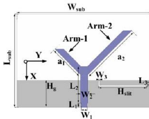
Figure 9 The geometry of the Y- shaped multiband CP antenna
