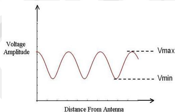
Figure 17 Voltage measured along a transmission line [27]
