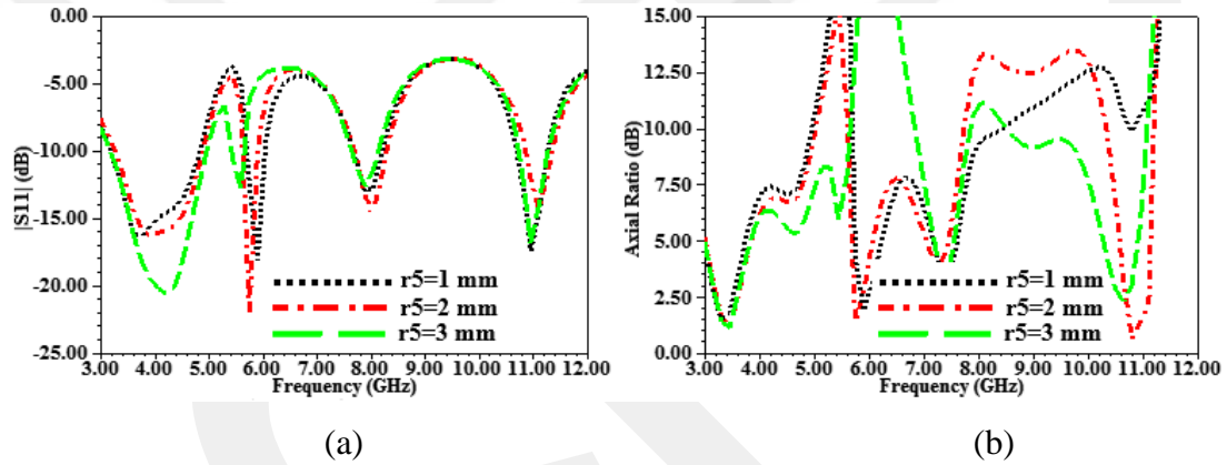
Figure 117 The effect of r_5 on second updated antenna performance (a) |S_{11}| , (b) AR
