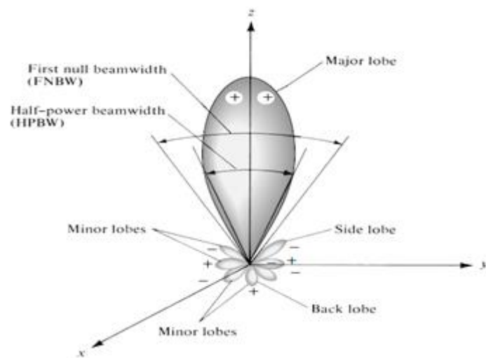
Figure 18 Radiation lobes and beamwidths of an antenna pattern [28]
