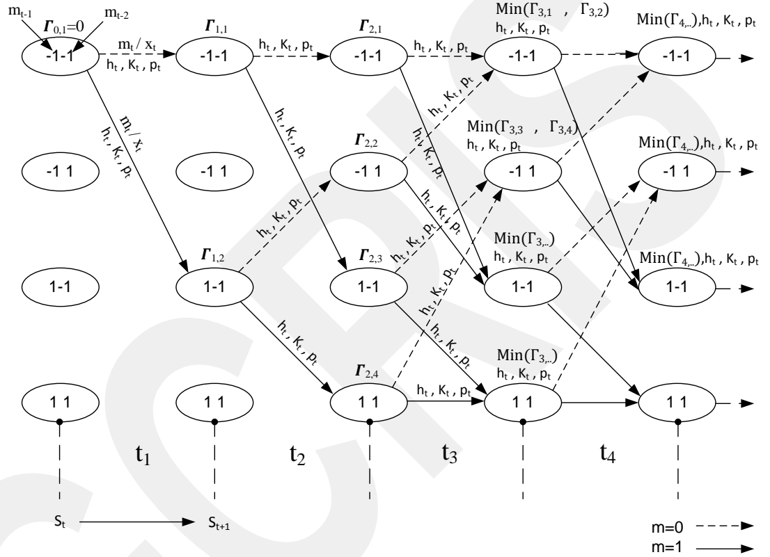
Figure 6: Viterbi RLS
