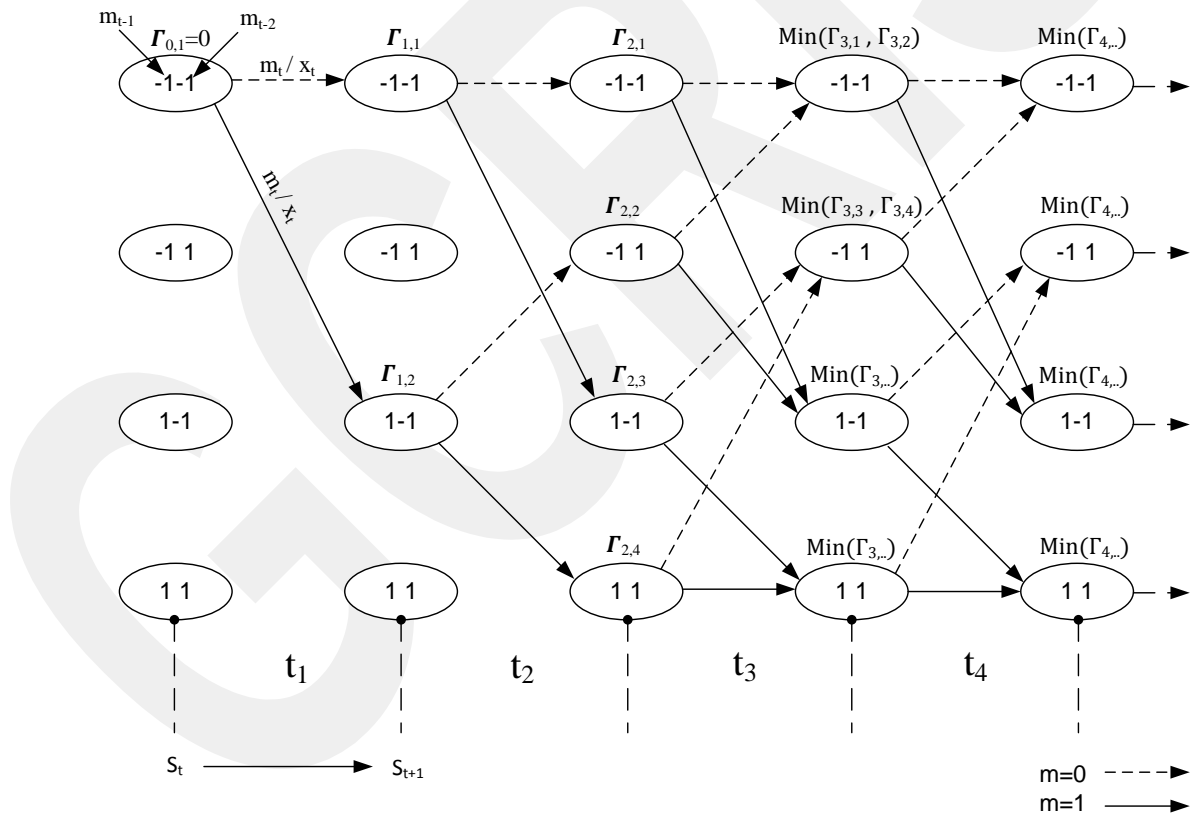
Figure 4: Viterbi MLSE
