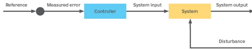
Figure 1.2: A Block Diagram of an Open Loop Control System [13]
