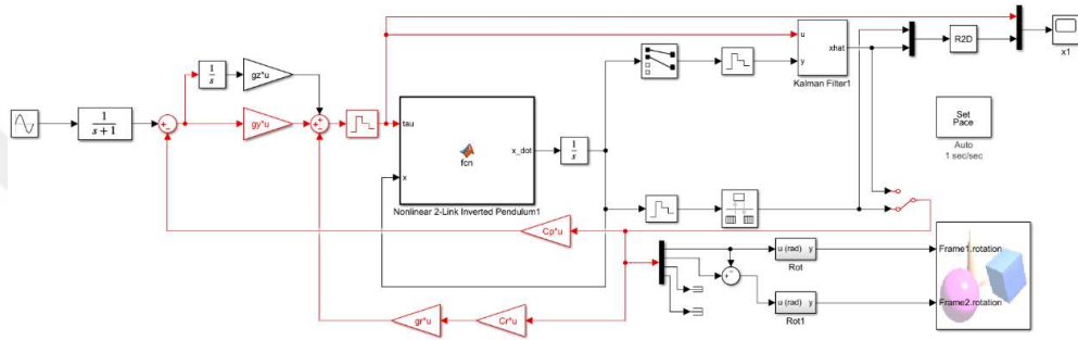
Figure 3.5: Simulink Diagram of the Simulation Process.
