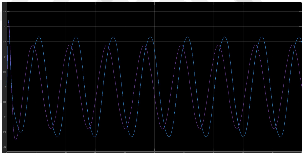
Figure 4.2: Difference between Simulated Data (Purple), and Kalman Approximation (Blue) of \dot{\theta}_2
