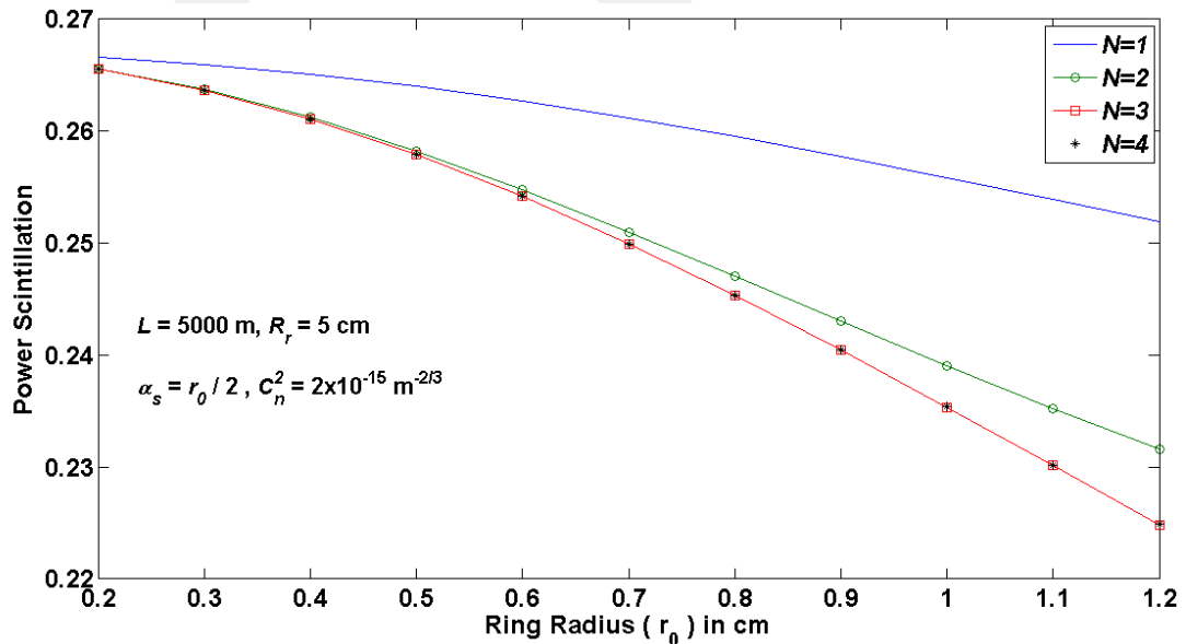
Figure 4 The power scintillation versus the ring radius r_0 assuming L = 5000 m, R_r = 5 cm, C_n^2 = 2 \times 10^{-15} \text{ m}^{-2/3} for different number of beamlets N and the source size \alpha_s values.
