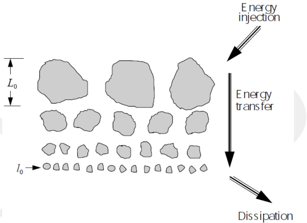
Figure 2 Kolmogorov cascade theory of turbulence.
