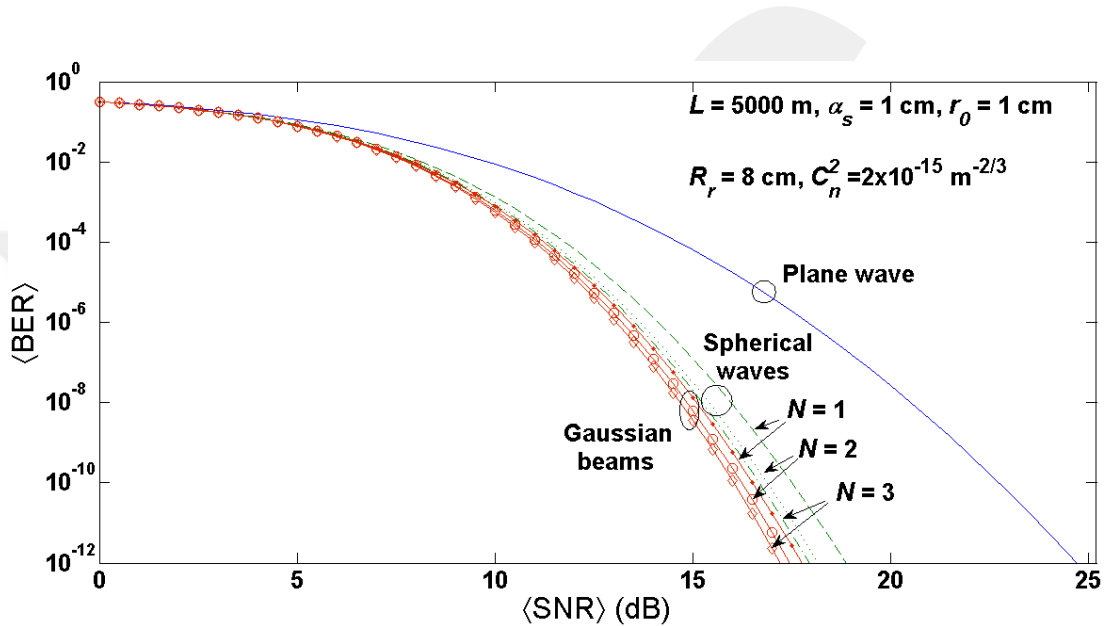
Figure 9 \langle \text{BER} \rangle comparison for plane, spherical and Gaussian waves.
