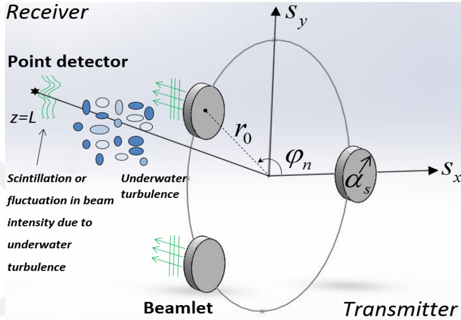
Figure 33 The illustration of MISO UWOC system with N=3 and formation of the scintillation.
