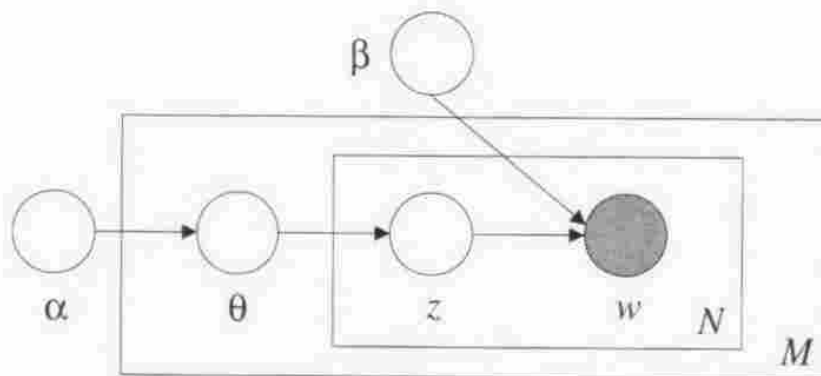
Figure-1: Graphical Model Representation of LDA from
