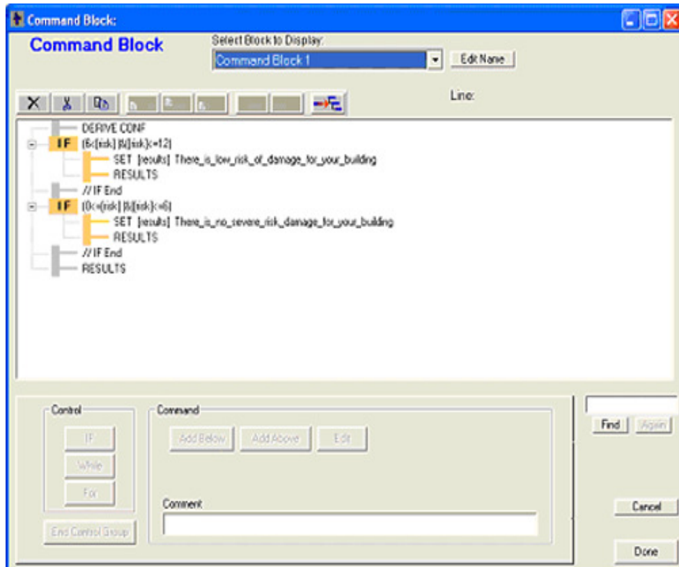
Figure 3.8. Building command block
