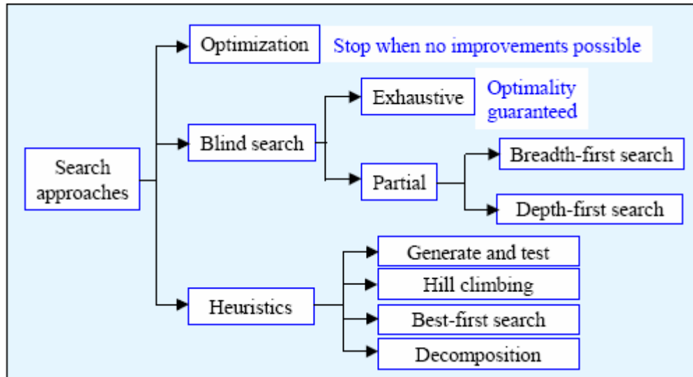
Figure 1.3. Search approaches.
