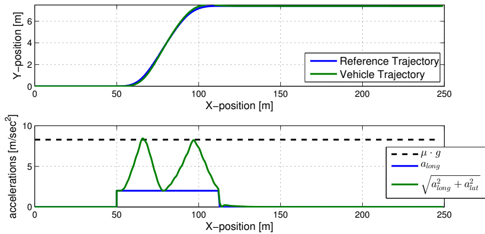
Figure 5.9: Trajectory following for v_0 = 20 m/sec, a_{\max} = 2 m/sec 2 , \mu = 0.82 and \Delta Y = 7.4 m.
