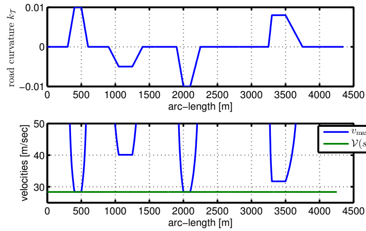
Figure 5.13: Road curvature (upper) and velocity comparison (lower) for v_{0.82} .
