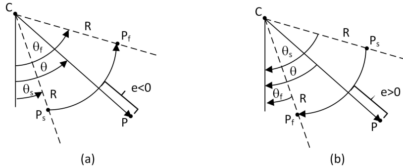
Figure 4.17: Distance error for an arc segment: (a) positive radius; (b) negative radius.
