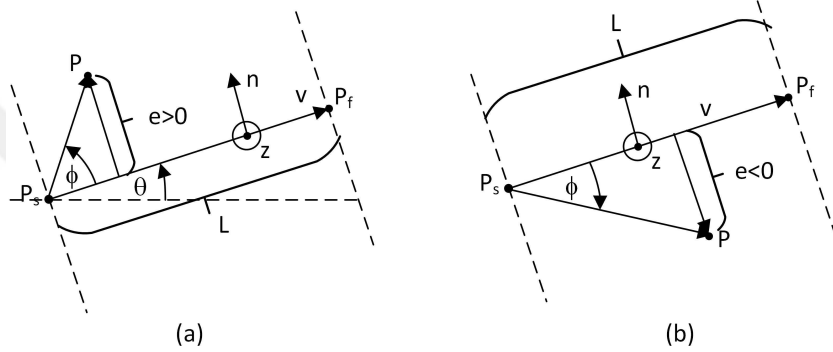
Figure 4.16: Distance error for a line segment: (a) positive error; (b) negative error.
