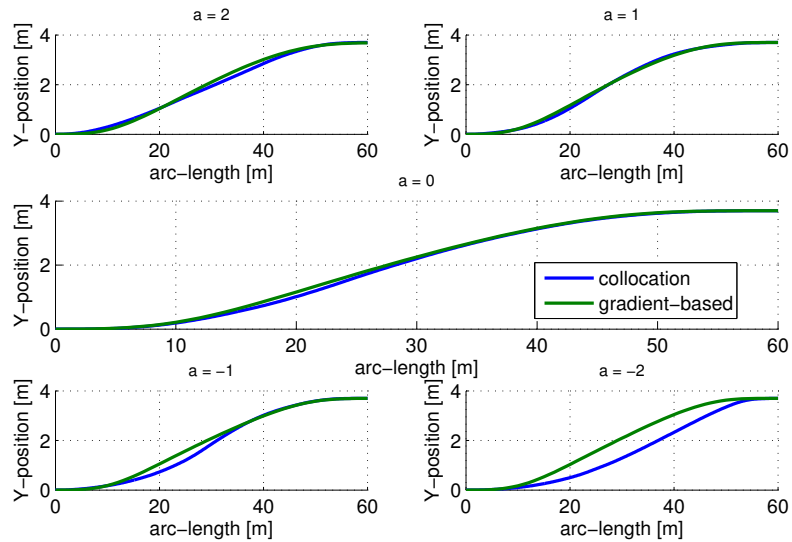
Figure 3.20: Comparison of optimal trajectories for S = 60 , v = 20 and a \in \{-2, -1, 0, 1, 2\} .
