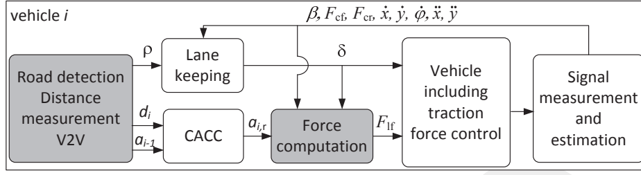
Figure 5.24: Control architecture for a generic vehicle i .
