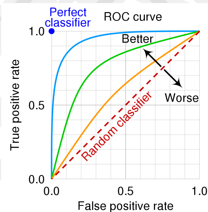
Figure 10 ROC Curve Example
