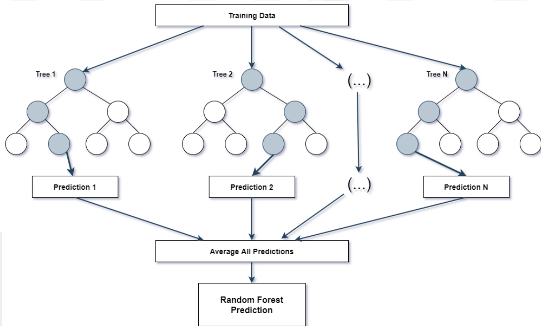
Figure 6 Random Forest Example
