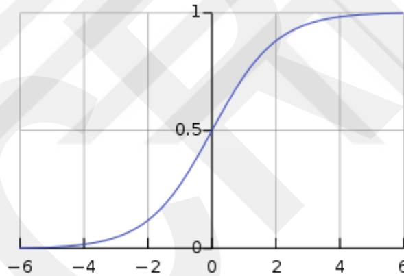
Figure 7 The Logistic Curve
