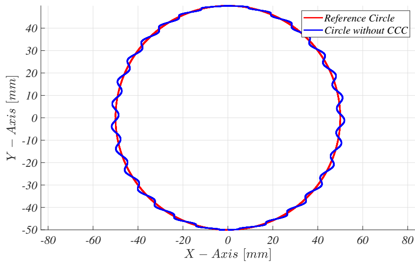
Figure 3.27: Drawing Circle under Inner Disturbance without CCC.
