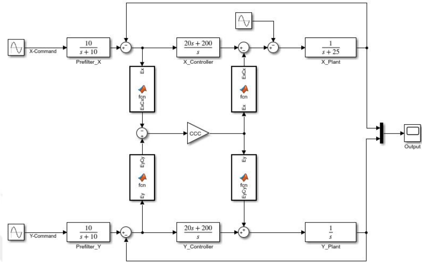
Figure 3.46: Block Diagram of Circle Drawing under Friction and Inner Disturbance.
