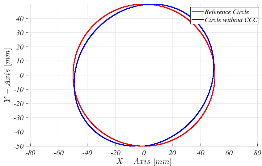
Figure 3.7: Drawing Circle under Friction without CCC.
