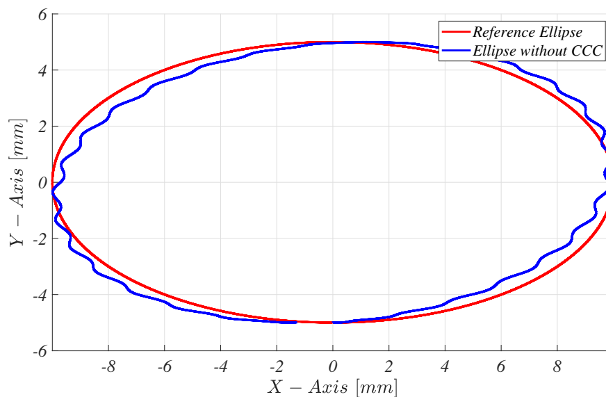
Figure 3.52: Drawing Ellipse under Friction and Inner Disturbance without CCC.
