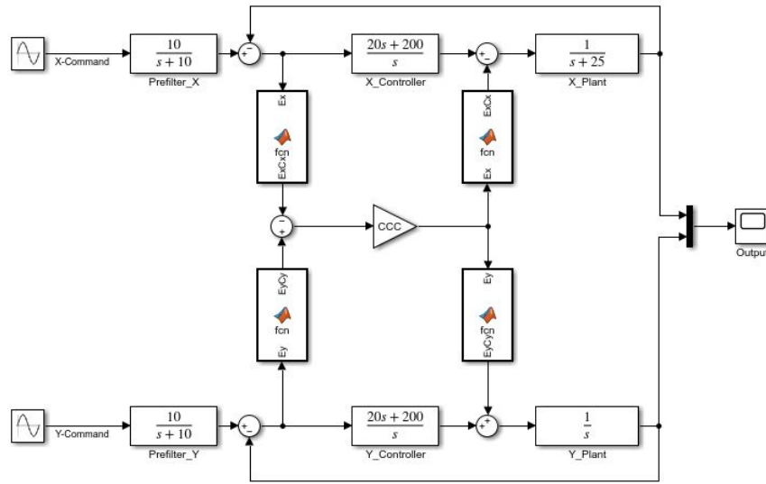
Figure 3.11: Block Diagram of Ellipse Drawing under Friction.
