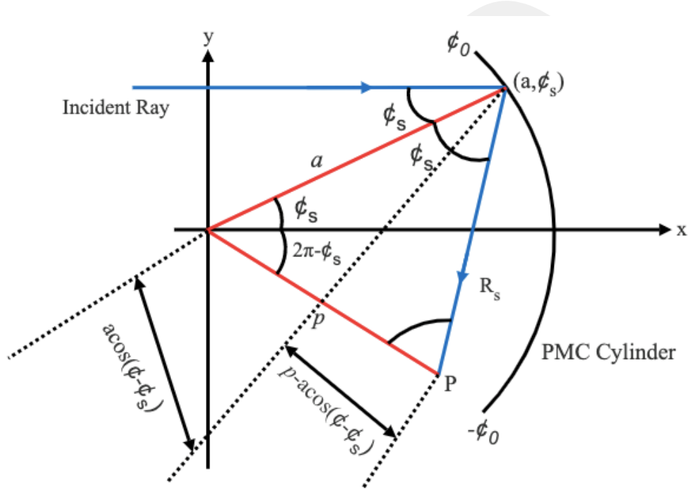
Figure 7 Stationary phase geometry of the reflected field
