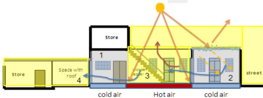
Figure 3.47: Ventilation and cooling 1; the two courtyards help air movement because courtyard 3 is sunny and courtyard 2 is shady.
