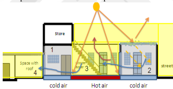
Figure 4.9: Ventilation and cooling by the courtyard; using two yards, one is shaded and the other sunny. Thus, different areas of pressure will help the cold air to move from the high- pressure areas to the low- pressure areas.
