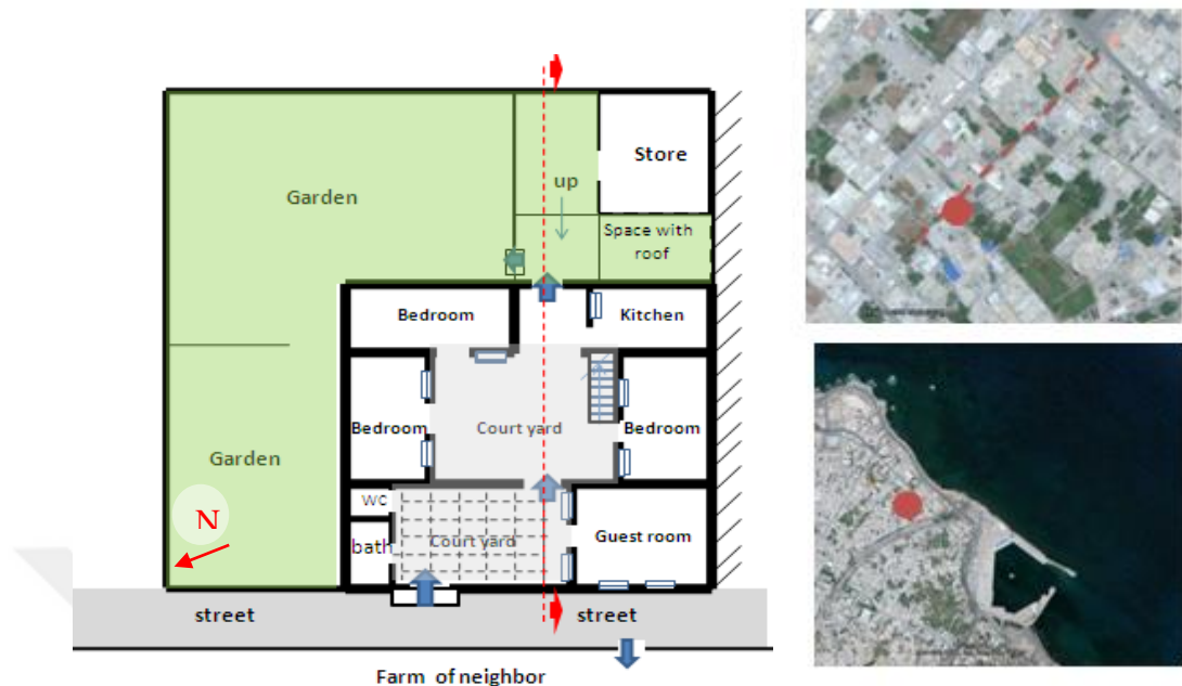
Figure 3.45: Plan and location of the housing
