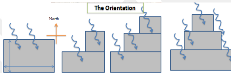
Figure 4.6; Ventilation and cooling; It is preferable that the building be facing the northwest wind without obstacles as it illustrates here
