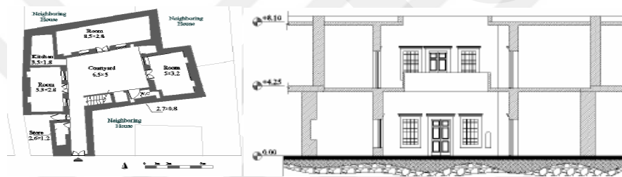
Figure 2.4: Traditional house in Tripoli, [22]
