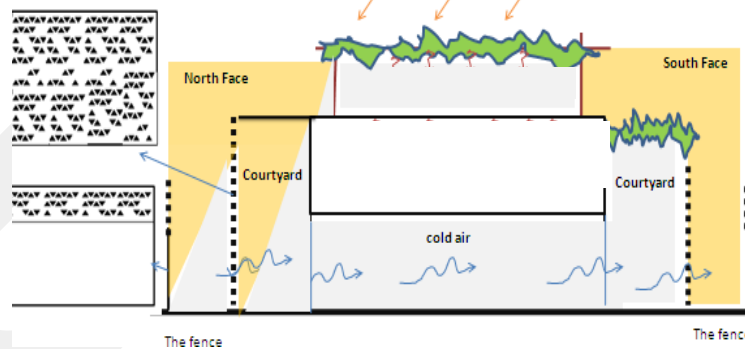
Figure 4.10: Ventilation and cooling by courtyard 2; covered wall allowing for shade and privacy. The green surface reduces solar heat and gives shade by dispersing light and radiation as well as absorbing solar radiation.
