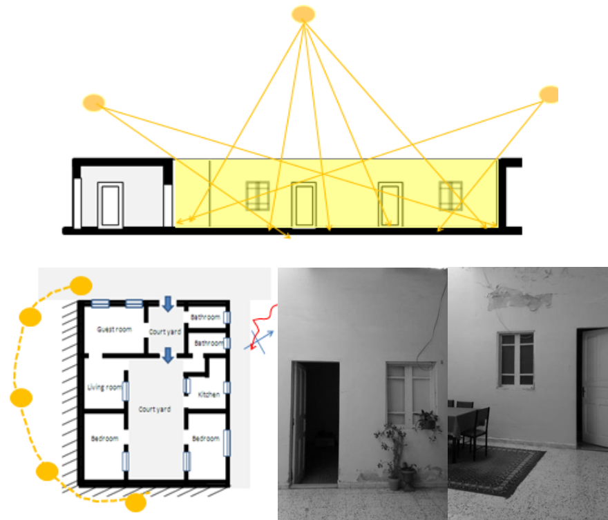
Figure 3.32: Lighting system; courtyard providing good light for every room
