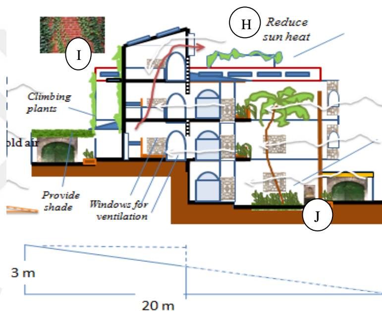
Figure 4.59; section the hall of the stairs works as wind catcher
