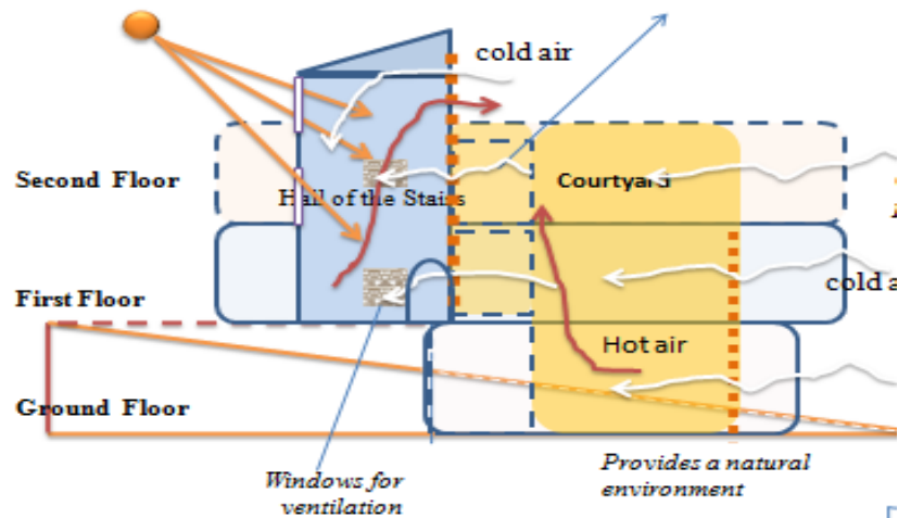
Figure 4.60; section analysis
