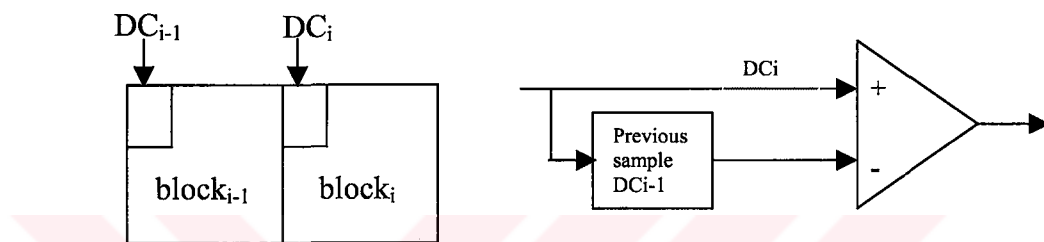
Figure C.3 Predictive Coding for DC coefficients
