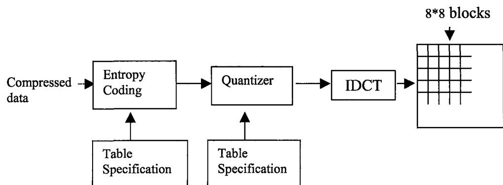
Figure C.4 JPEG Decoder
