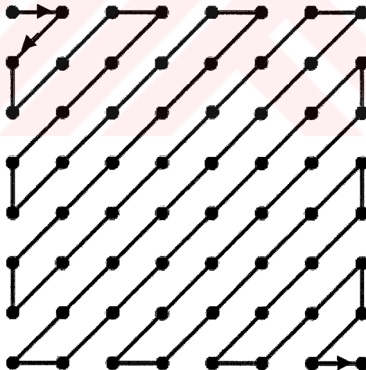
Figure C.2 Zigzag Scan
