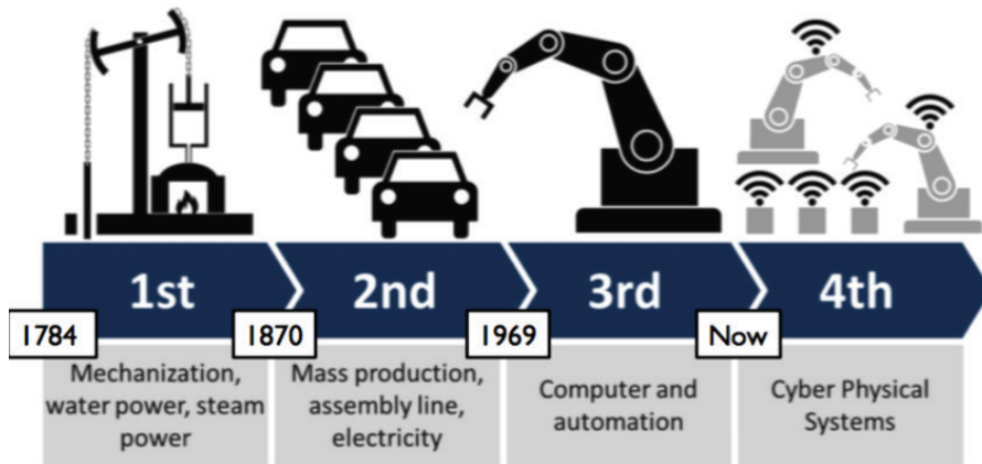
Figure 1: Industrial Revolutions
