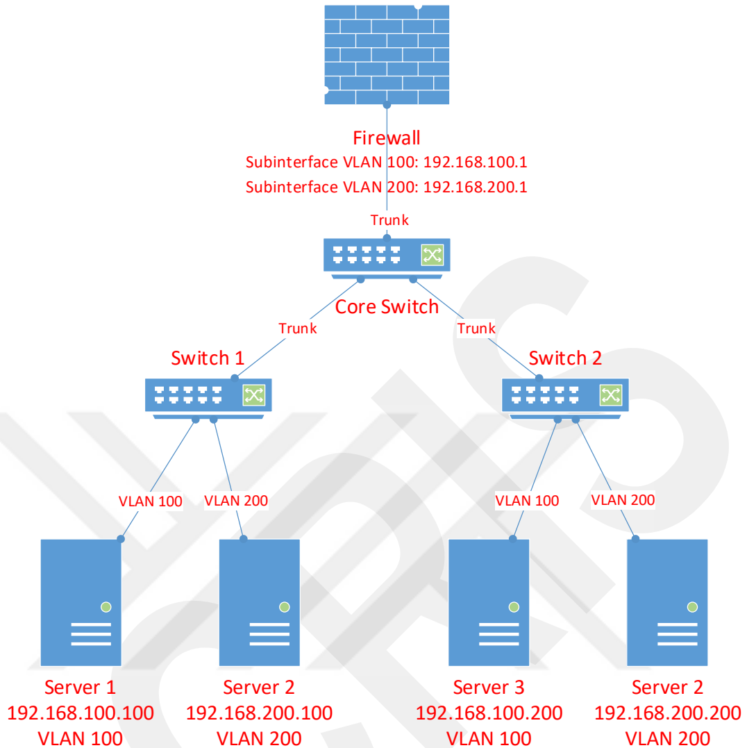
Figure 7: General firewall placement in traditional networks
