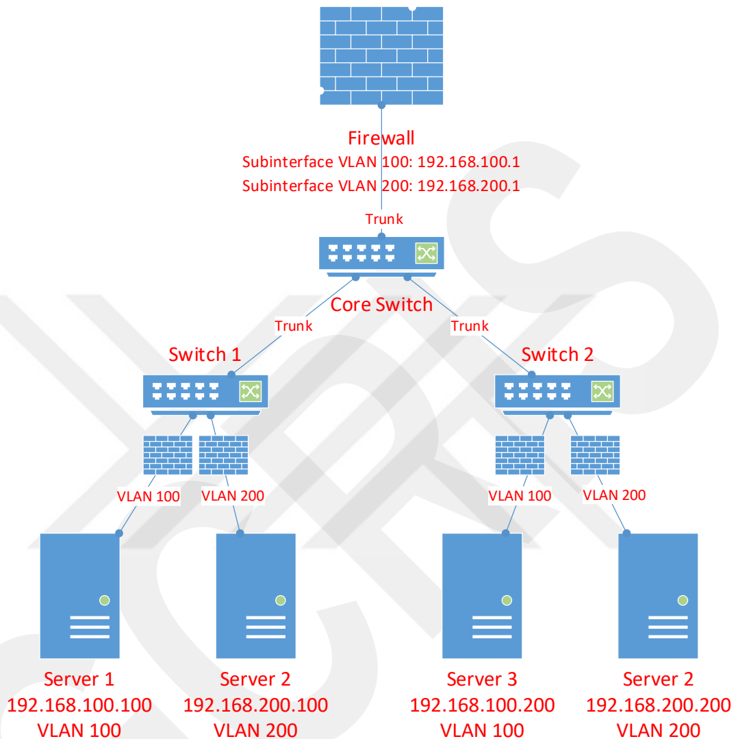
Figure 8: Firewall placement in a virtualized environment
