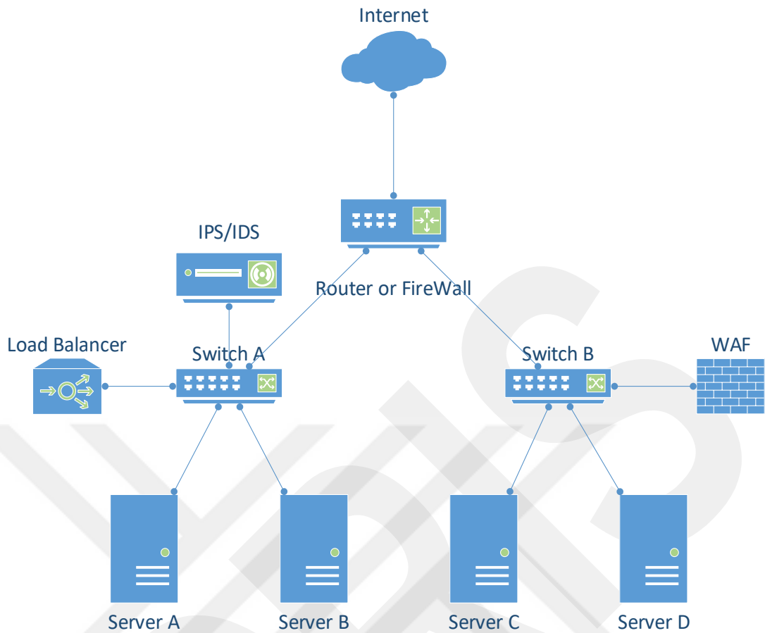
Figure 4: Simple traditional network infrastructure
