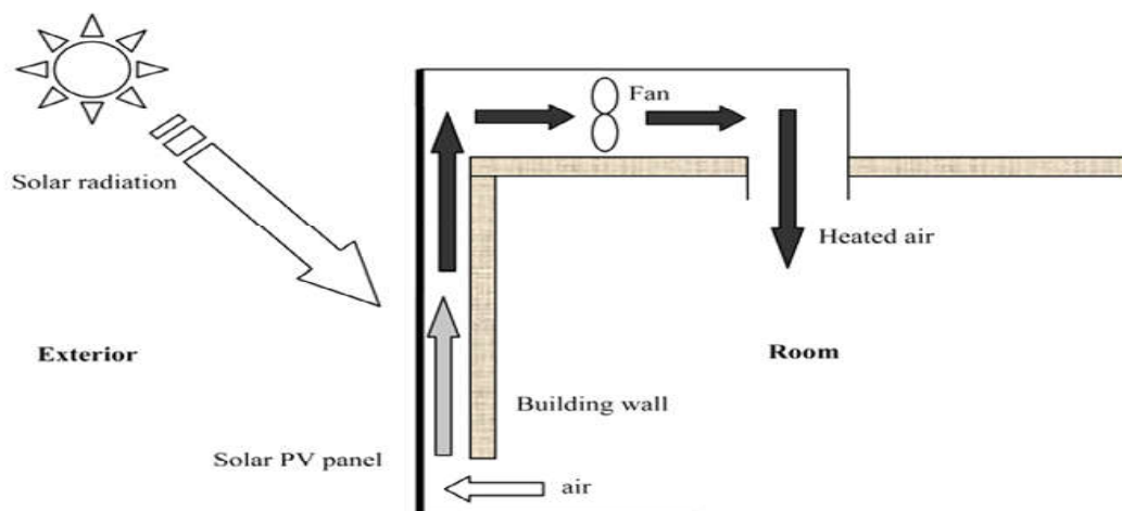
Figure 2.7: Schematic Illustration of a BIPVT System[43]
