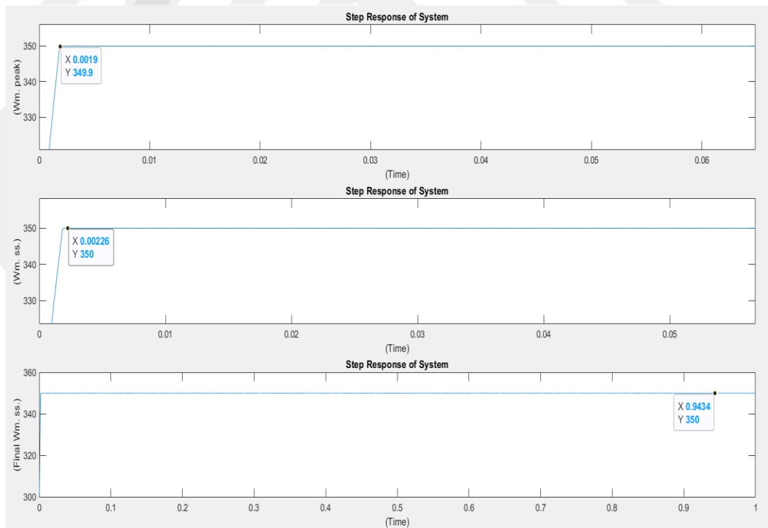
Figure 45: FLC (GA) (Multiple) 300-350 (Wm_peak(rad/sec): 349.9, tr (sec.): 0.0019, Wm_ss(rad/sec): 350, ts (sec.): 0.0022, Final Wm_ss(rad/sec): 350)
