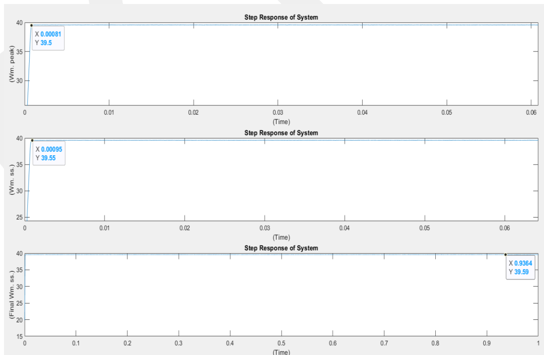
Figure 72: FLC (GA) (Multiple) Norm 1 (20)-(40) (Wm_peak(rad/sec): 39.5, tr (sec.): 0.00081, Wm_ss(rad/sec): 39.55, ts (sec.): 0.00095, Final Wm_ss(rad/sec): 39.59)
