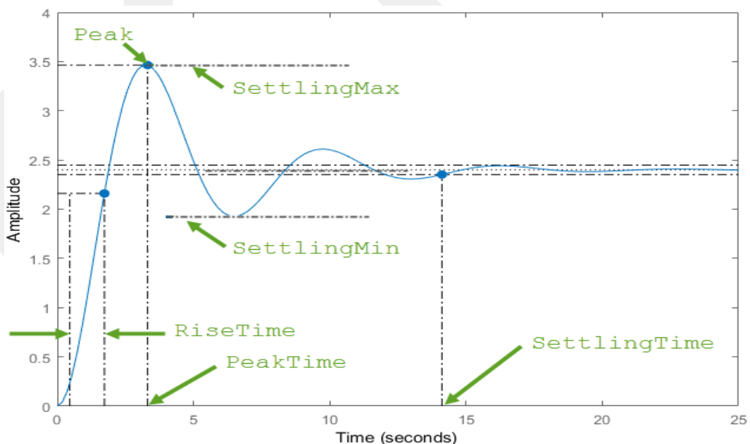
Figure 8: Step Response [16]
