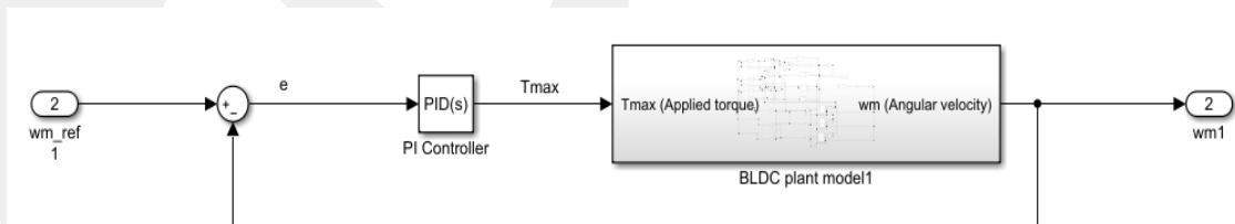
Figure 6: Closed loop PI control for the angular speed of the BLDC Motor
