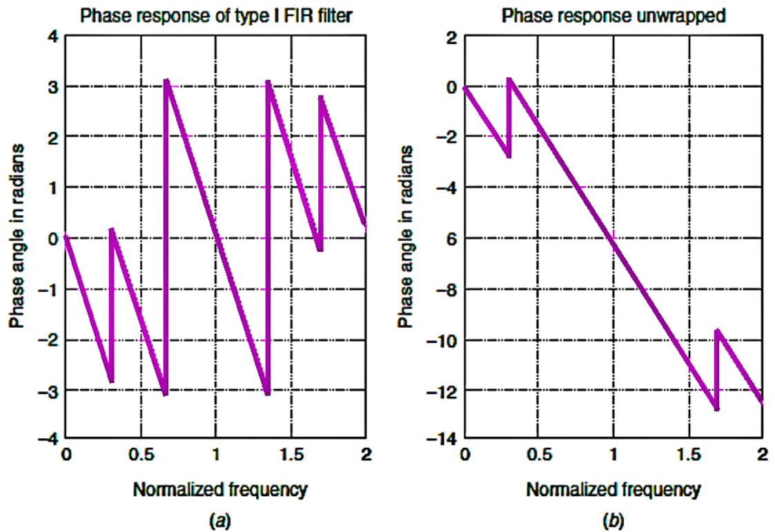
Figure 10 Linear Phase Responses of Type I FIR Filter
