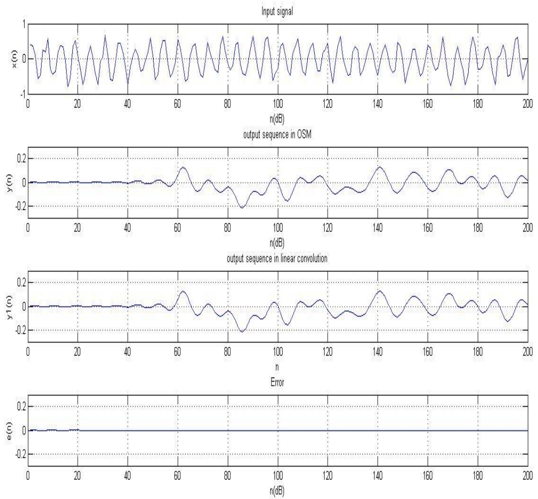
Figure 29 Comparison between OSM method and the linear convolution
