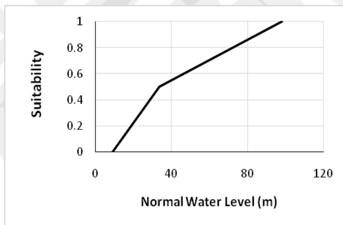
Figure 23 Suitability function for the normal water level (head) criterion
