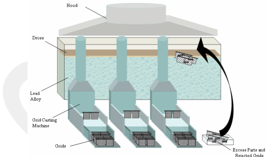
Figure 5.23 Representation of Batch Addition of Excess Parts and Rejects
