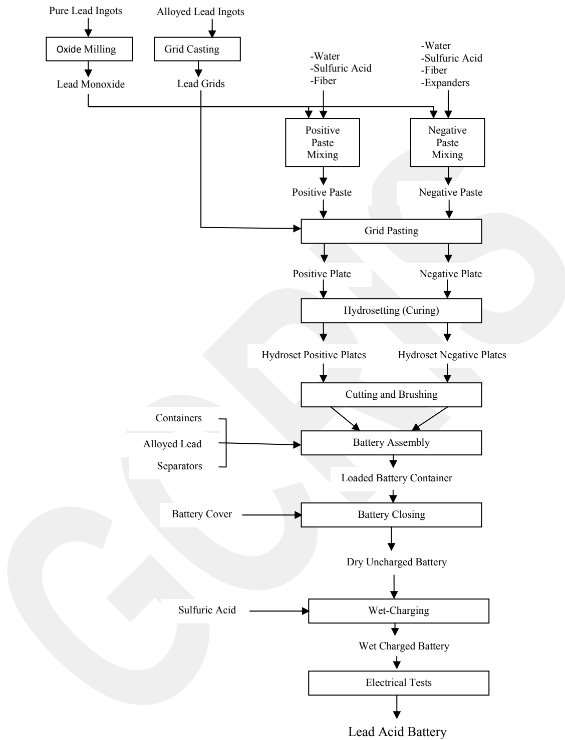
Figure 5.7 Manufacturing Scheme of a Lead-Acid Battery
