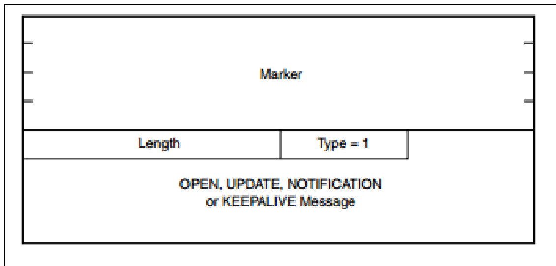
Figure 7. BGP Header [2]
