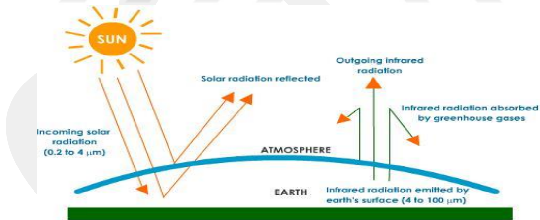
Figure 2.1: Simplified diagram illustrating the greenhouse effect (Change, 1998)
