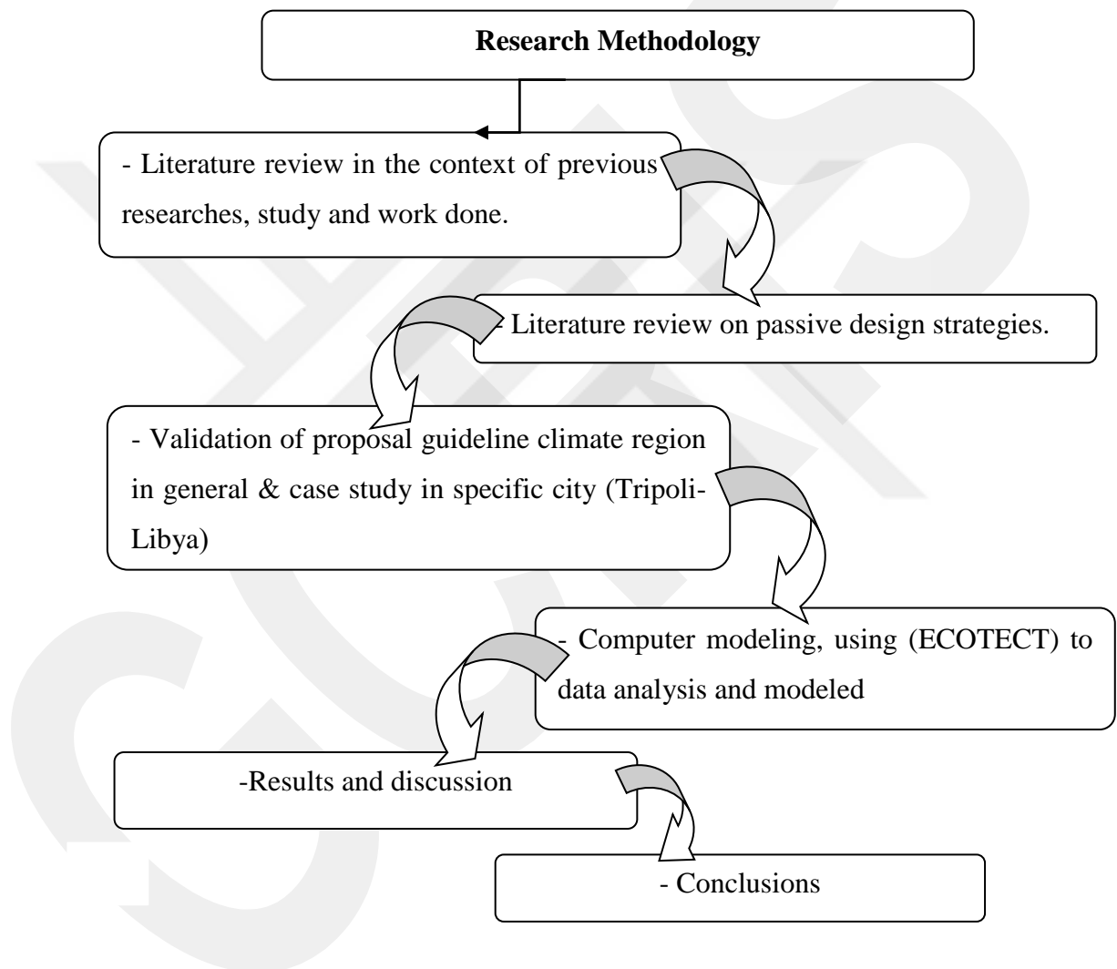
Figure 1.1 Research methodology
