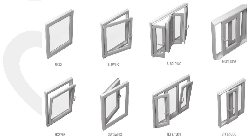
Figure 3. 17: Types of Operable Windows (tiltco.net)
