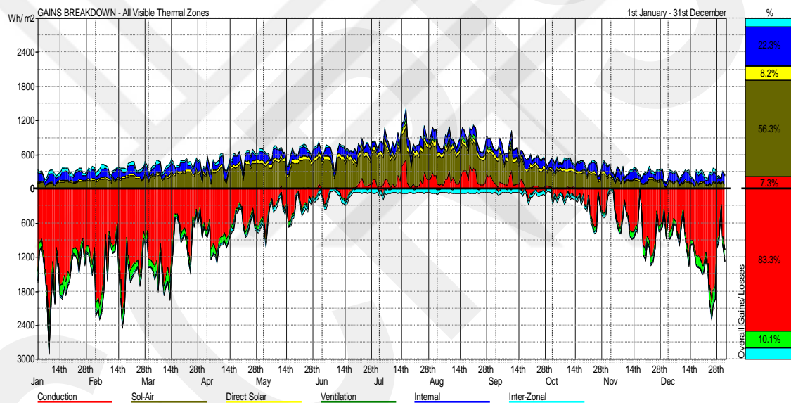
Figure 4. 6: passive gains and losses on ECOTECT simulation when using the materials mentioned as Alternative 1 (Table 4).
