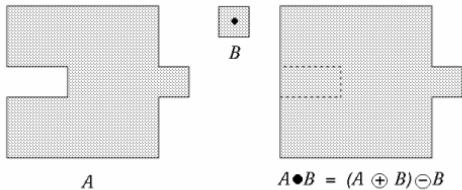
Figure 3.8: Closing operation
