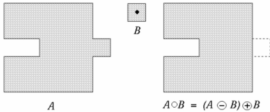
Figure 3.7: Opening Operation
