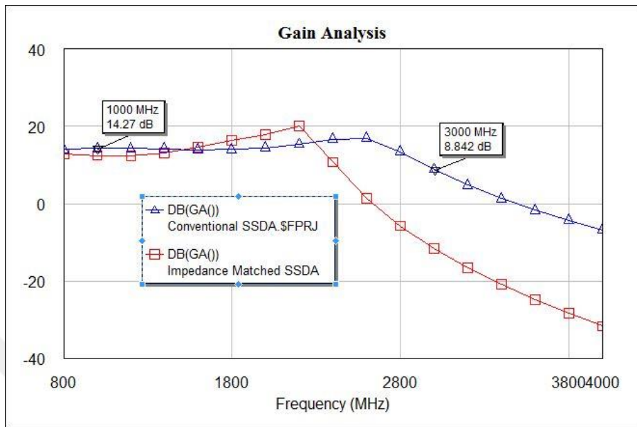
Figure 32 Available gains of SSDA and impedance matched SSDA
