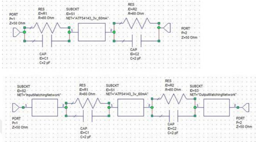
Figure 7 WithImpedanceMatching and WithoutImpedanceMatching circuit schematics
