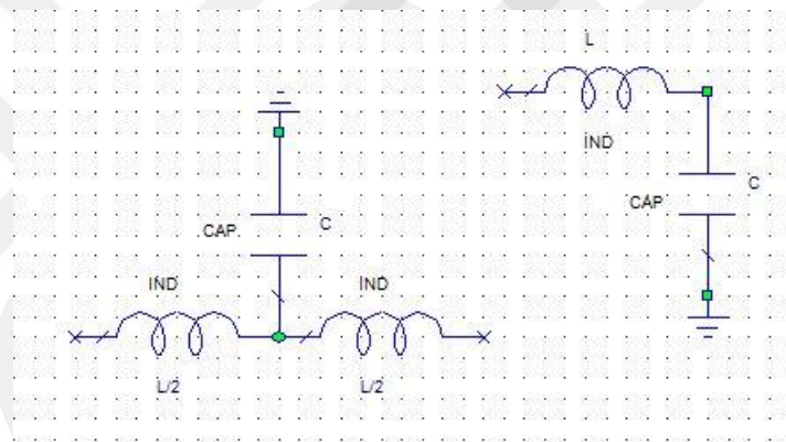
Figure 24 Basic schematics of T type and L type artificial transmission lines [25]
