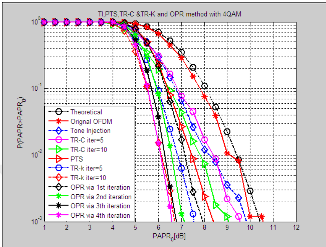
Figure 30 Simulation results of the PAPR techniques employing 4-QAM.
