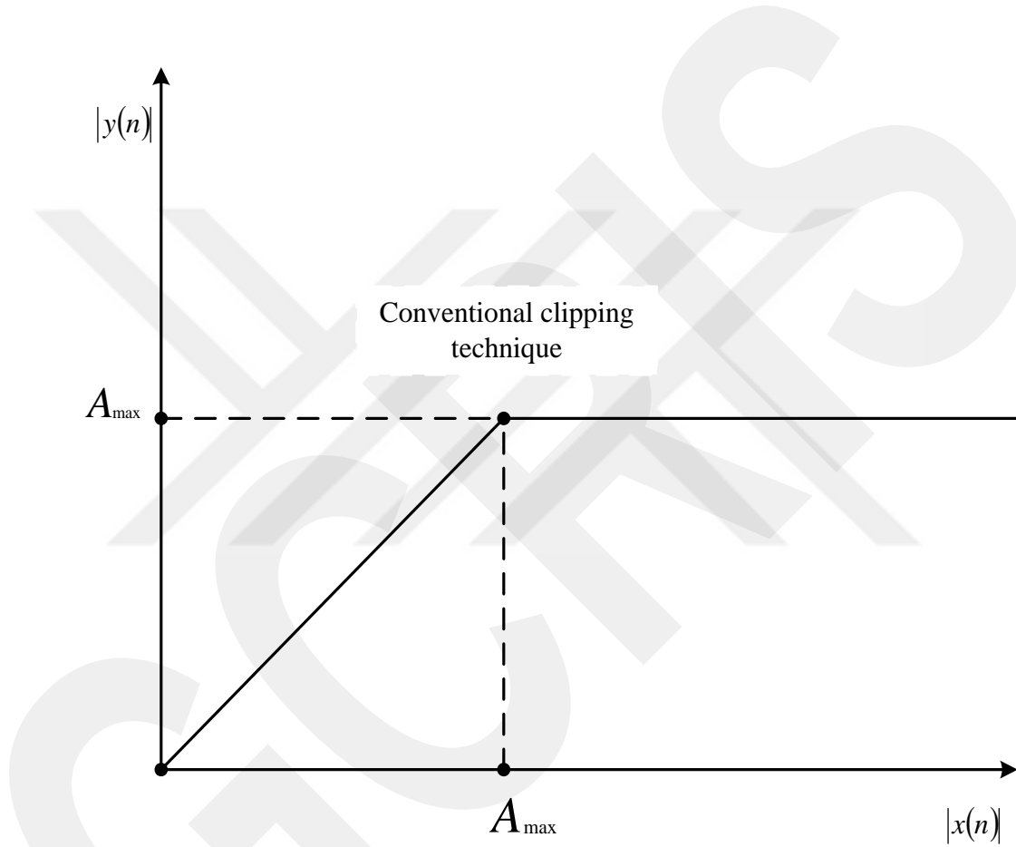
Figure 14 Classical amplitude clipping function [26]
