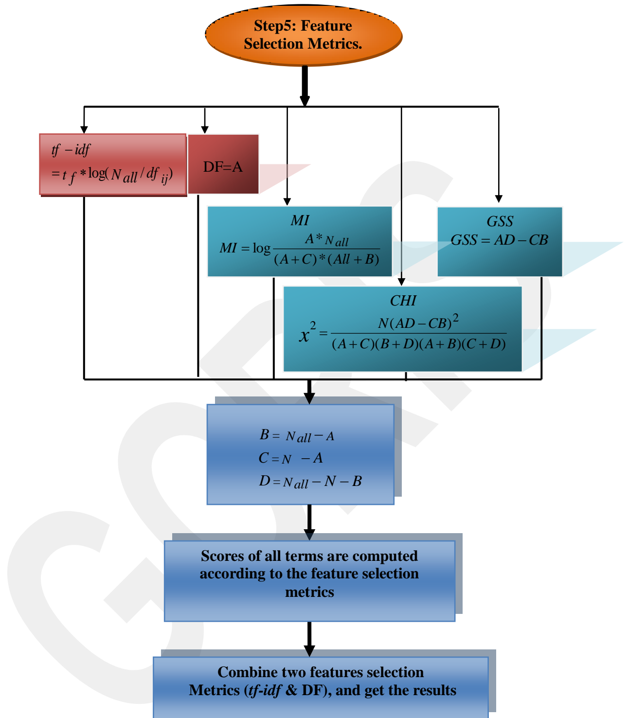
Figure 9 Feature Selection Metrics.
