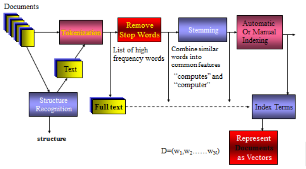
Figure 4 The Document Preprocessing Chart.
