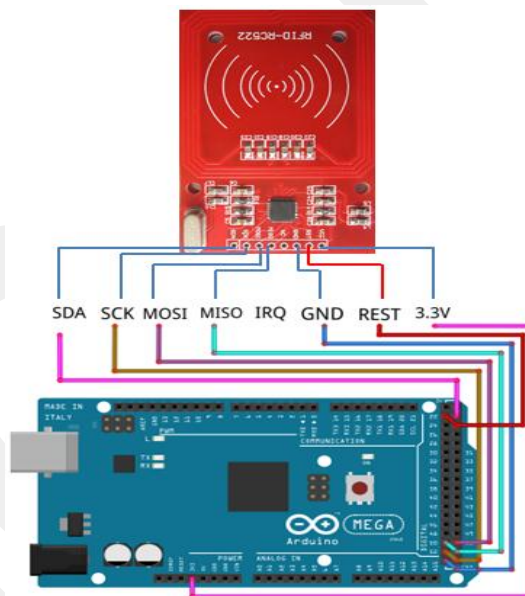
Figure 35: Block diagram of the RFID with the Arduino
