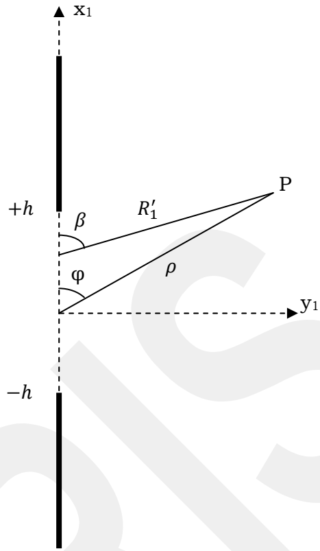
Figure 3.2. Geometry of the impedance slit.
