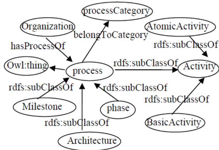
Figure 11: Process Experiences Ontology [28]
