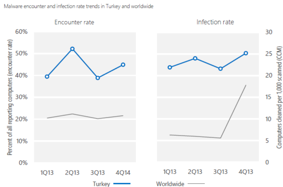
Figure 4 Malware encounter and infection rates in 2013
