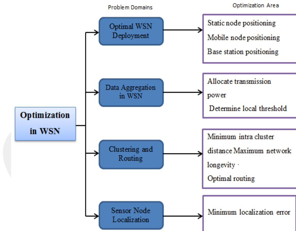
Figure 16 Optimization domains in WSNs
