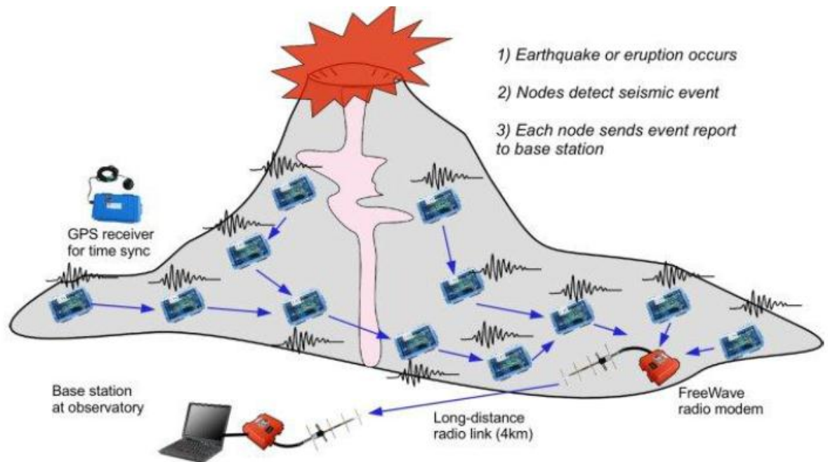
Figure 9 Implementation of WSN in Detection of Volcanic Activity [10].
