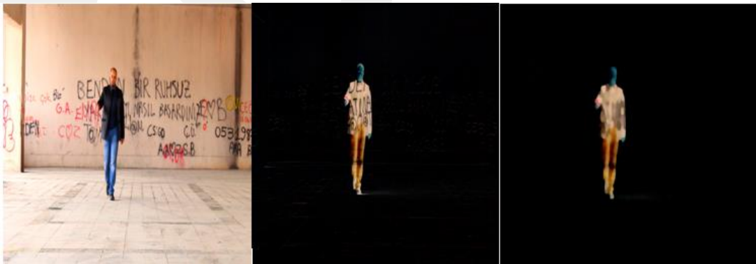
Figure 5: Morphological operations.
