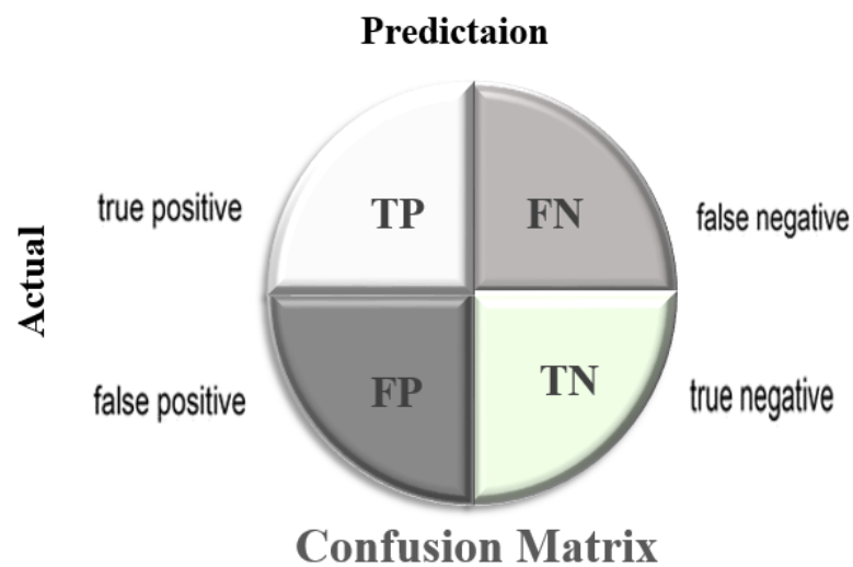
Figure 40: Confusion Matrix.
