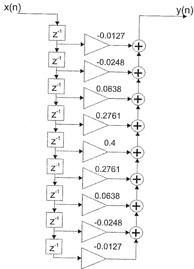
Figure 8 FIR filter realization
