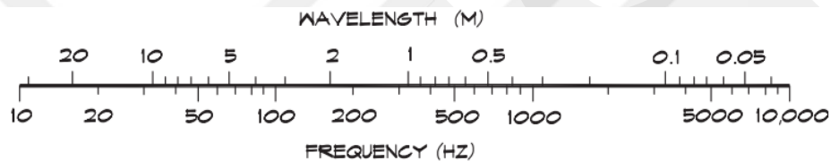
Figure 2.2. Wavelength versus Frequency in air at 20° (Harris, 1992; cited in: Long, 2006)
