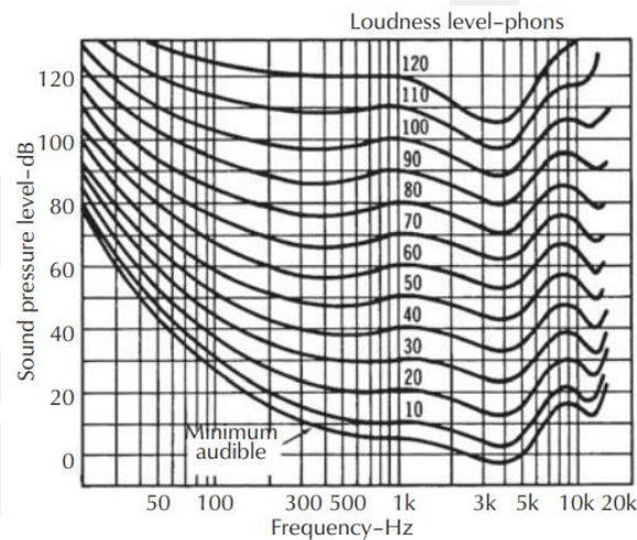
Figure 2.11. Equal loudness contours for pure tones in the frontal sound field for humans of average hearing acuity. The loudness levels in phons correspond to the sound pressure levels at 1kHz (Ballou, 2008)
