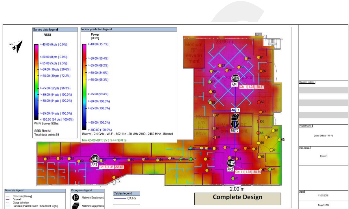
Figure 7: Fastray Path Loss Propagation Model
