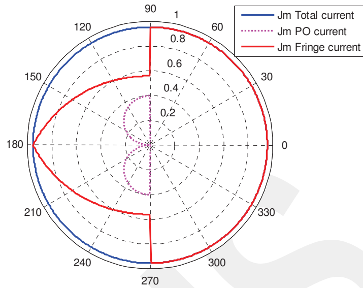
Figure 15 Magnetic currents flowing on impedance cylinder for small radius
