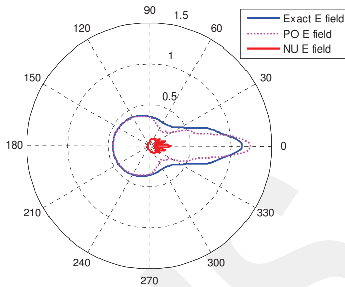
Figure 17 Scattered electric fields from PEC cylinder
