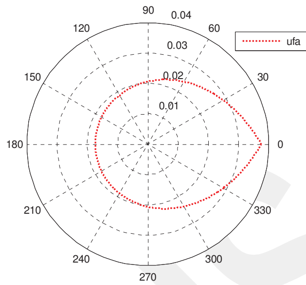
Figure 29 The asymptotic fringe field when \sin \theta \rightarrow \infty
