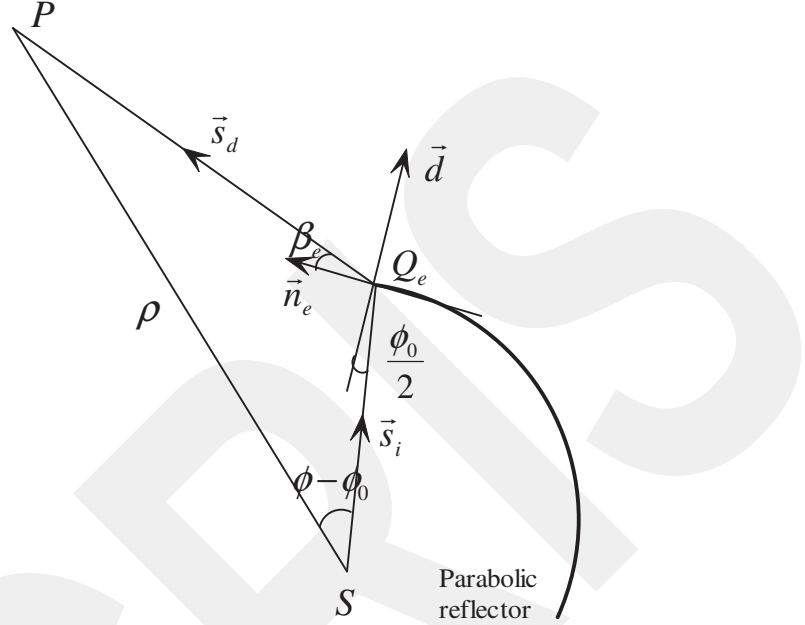
Figure 23 The geometry of diffracted fields
