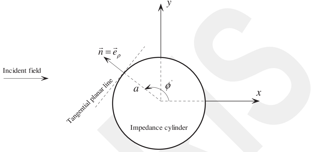
Figure 8 The impedance cylinder geometry
