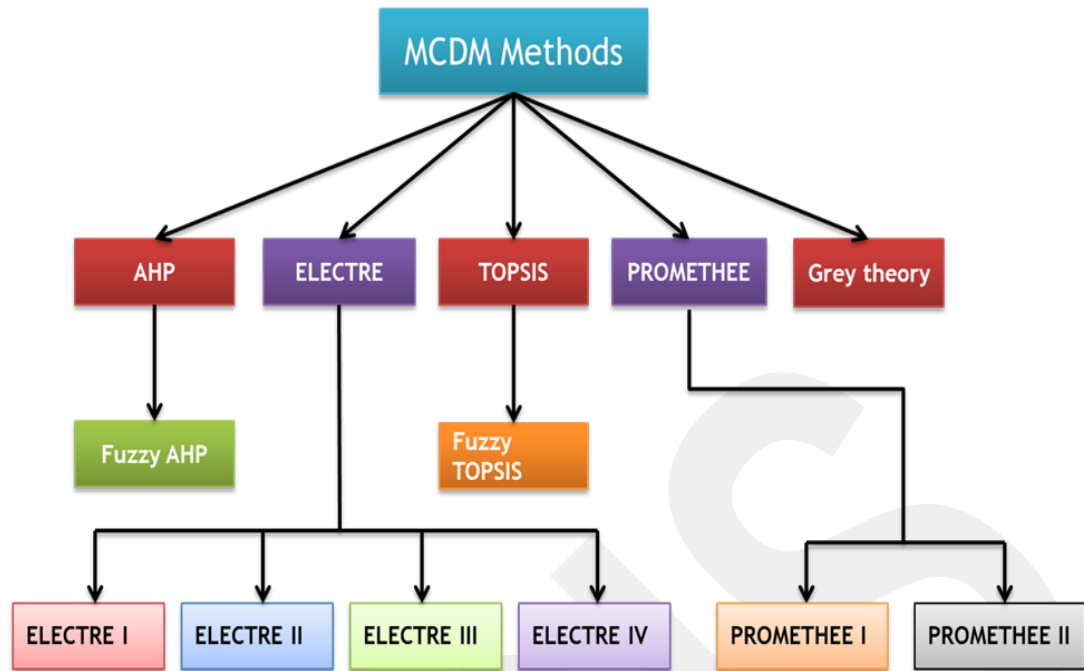
Figure 4.2 : Hierarchical Structure of MCDM Methods
